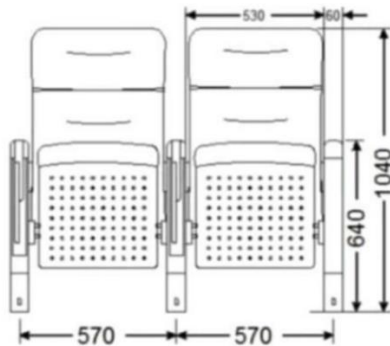
Figure 2: Front View Dimension of Chair
