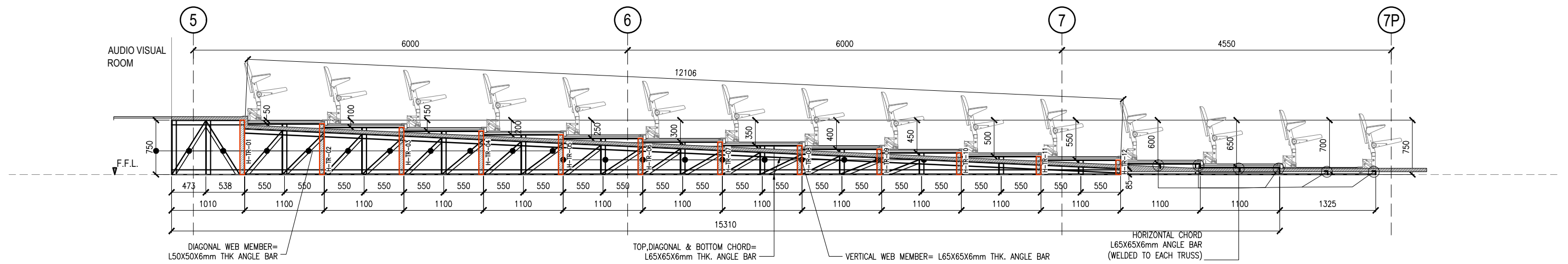
TRUSS-05
