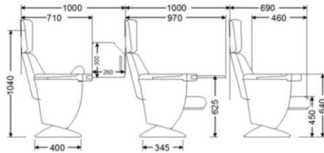
Figure 1: Side View Dimension of Chair
